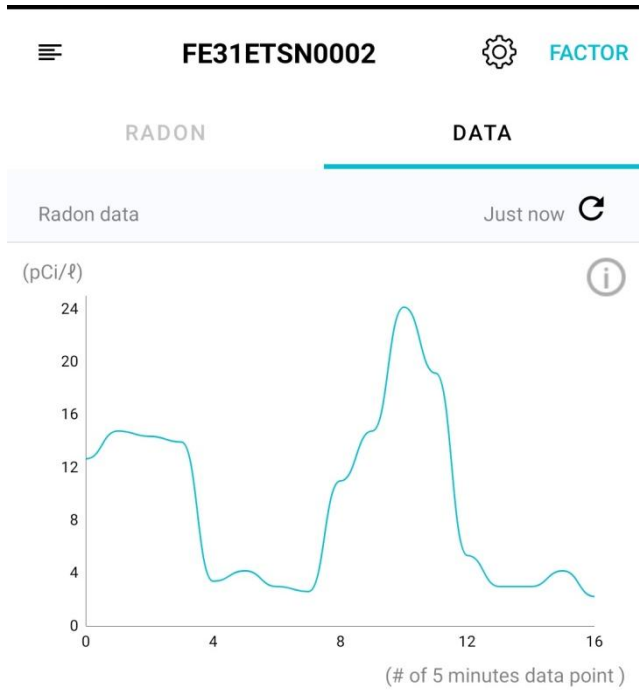
Figure 22: Graph of Ecotracker #02 results in a 19.2 pCi/l Chamber for 20 minutes and then outdoors for 20 minutes then in the chamber for 20 minutes and then outdoors for 20 minutes
