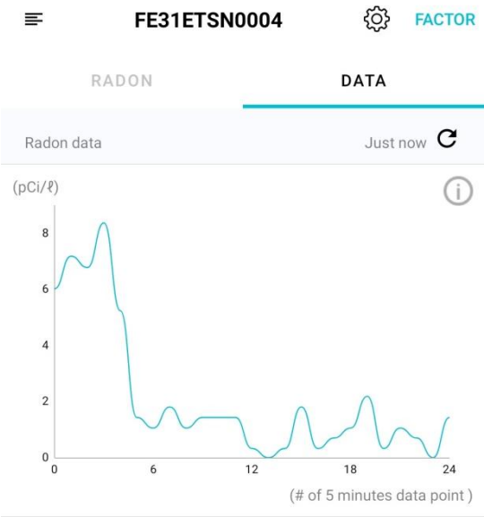
Chart 7: EcoTracker Low-level sniff test
