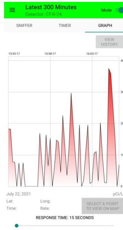
Figure 15: Graph tab displaying 15 second results for 19 pCi/l Chamber sampling
