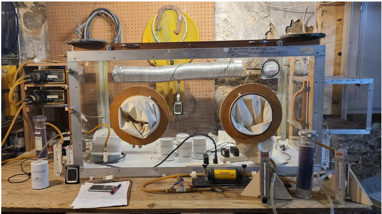
Figure 12: Radon Chamber
