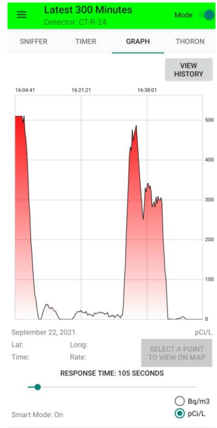
Figure 44: CT007-R Thoron and Radon chamber measurement
