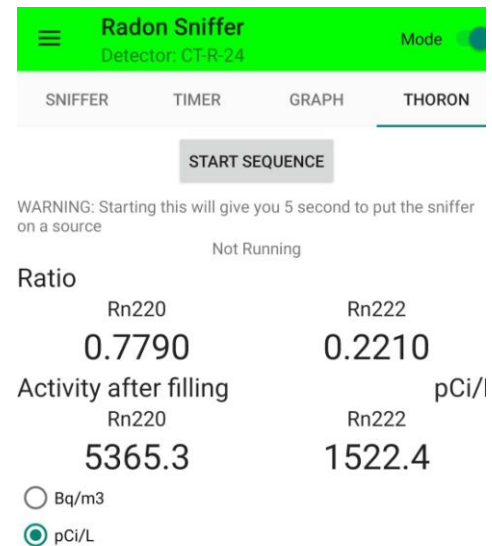
Figure 7: Thoron function
