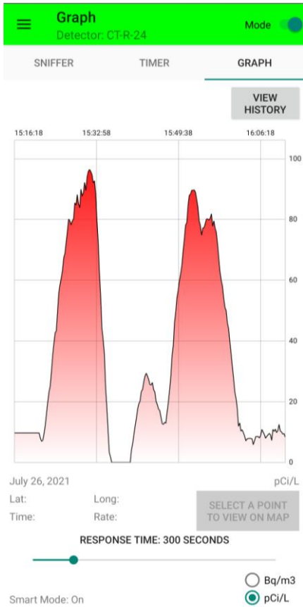
Figure 19: Graph displaying 300 second results over about 54 minutes
