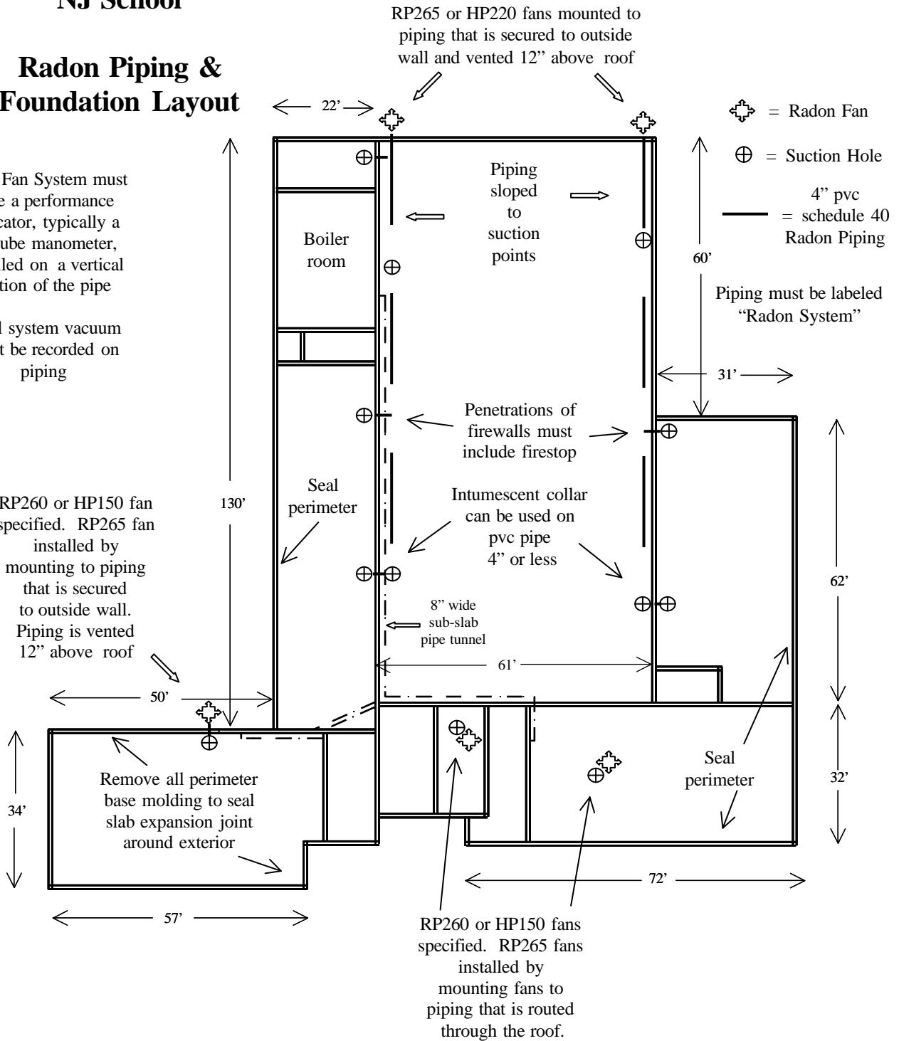
Figure 2. Foundation plan showing sub-slab divisions and final radon re-mediation piping and fan locations. Total interior perimeter and visible expansion joints sealed.
